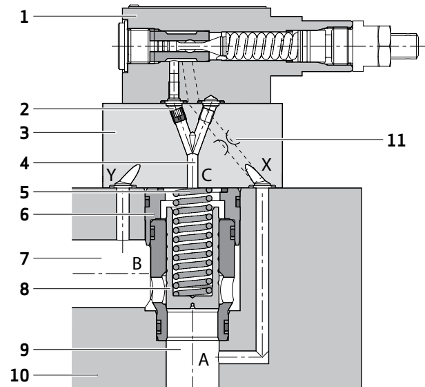
Pressure Cartridge Valve and Cover
