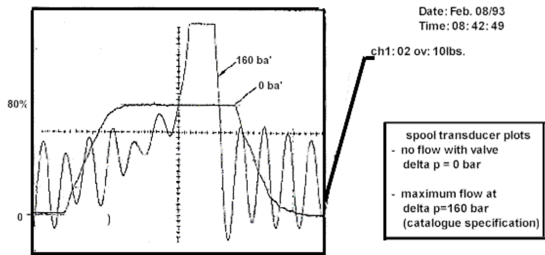
Figure 4: Step response of CETOP5 proportional solenoid value
