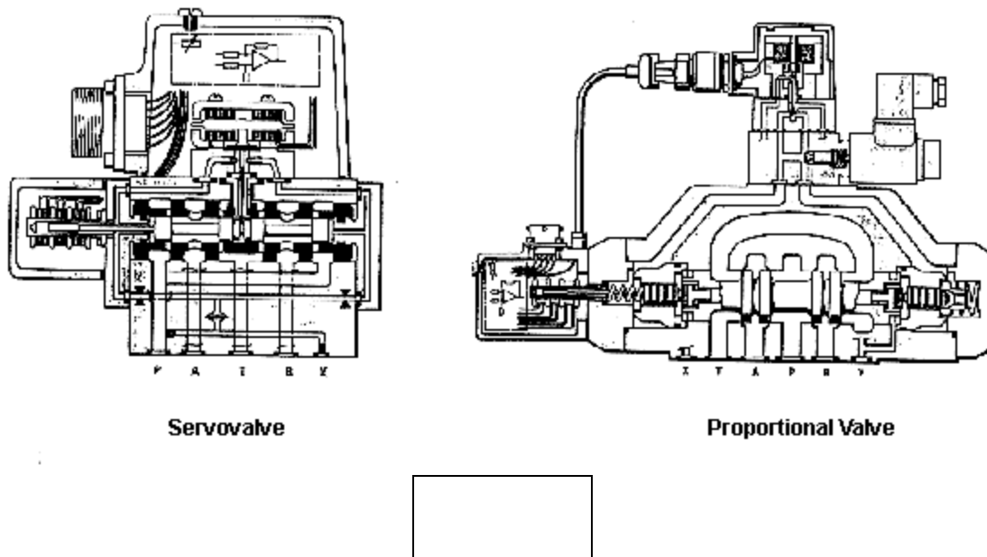
Figure 6: Electrical feedback valves
