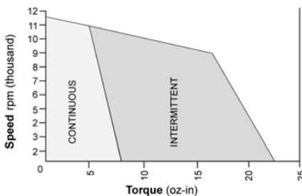
BN12-28AF-01: Continuous & Intermittent Operation at 12 Volt DC
