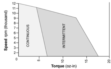
BN12-23AF-03: Continuous & Intermittent Operation at 36 Volt DC
