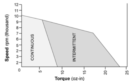
BN12-28AF-03: Continuous & Intermittent Operation at 36 Volt DC
