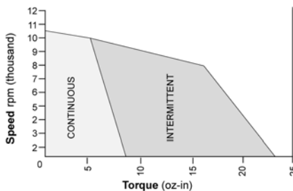
BN12-28AF-02: Continuous & Intermittent Operation at 24 Volt DC
