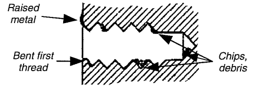
UNACCEPTABLE Conditions in Threaded Holes
