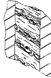
Potentially loose friction welded particles
