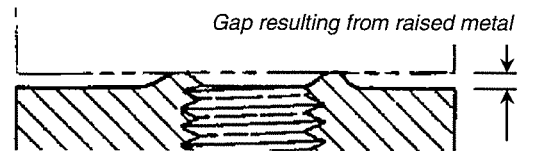
Extruded Material Surrounding Threaded Hole UNACCEPTABLE
