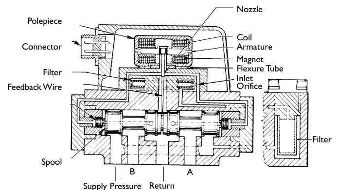
Figure 1 Moog Series 72K and (G)72K
