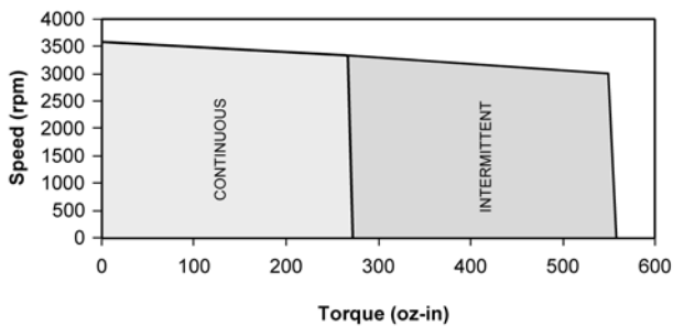
BSG34-38AC-01LH: Continuous & Intermittent Operation at 24 Volt DC
