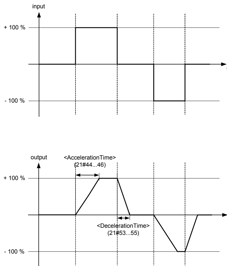
Figure 44: Ramp type 2
