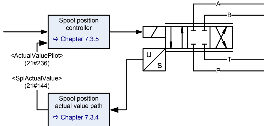
Figure 52: Single stage servo valve
