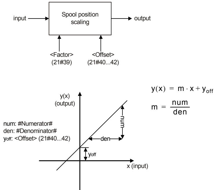
Figure 41: Scaling function
