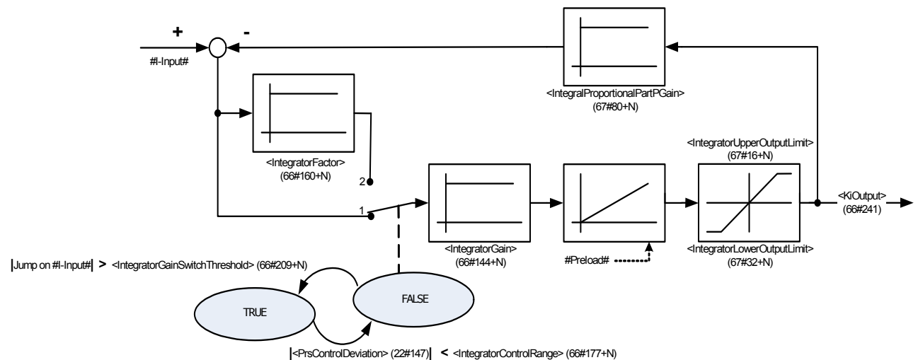
Figure 68: Integrator element (I)
