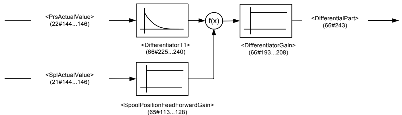
Figure 70: Derivative element (PD)
