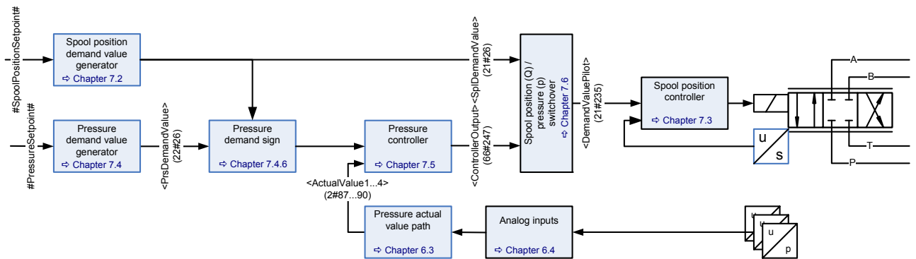
Figure 38: p/Q control closed loop
