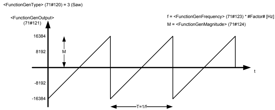
Figure 92: Sawtooth signal (type 3)
