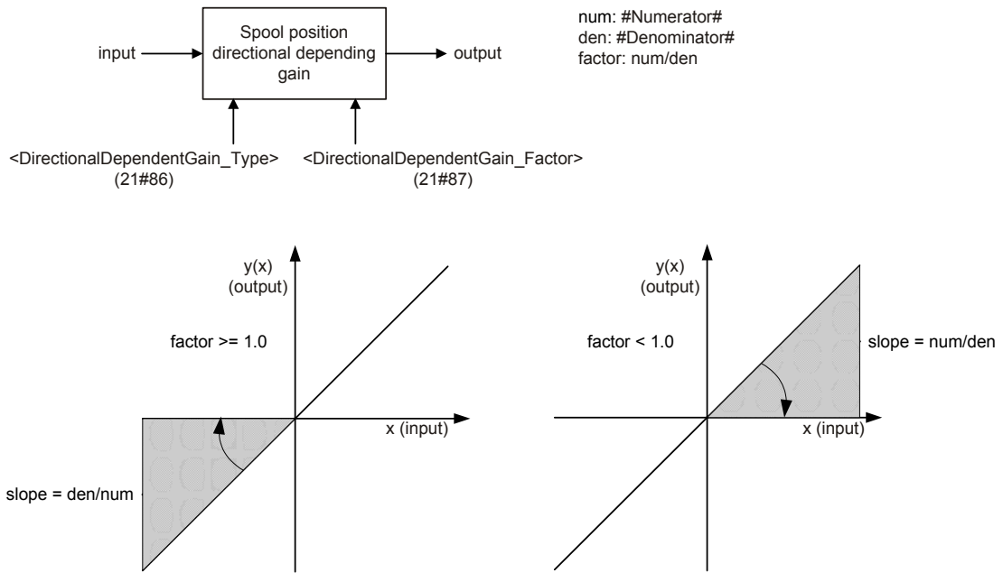
Figure 46: Directional depending gain
