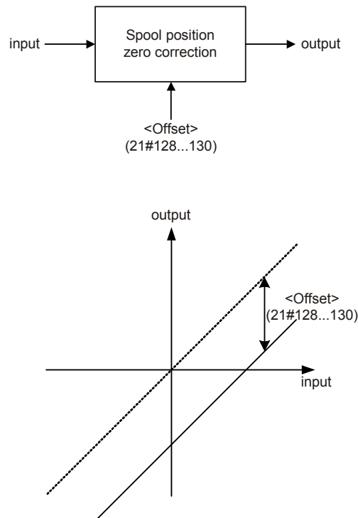
Figure 51: Zero correction
