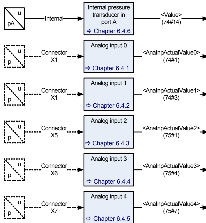
Figure 23: Analog inputs
