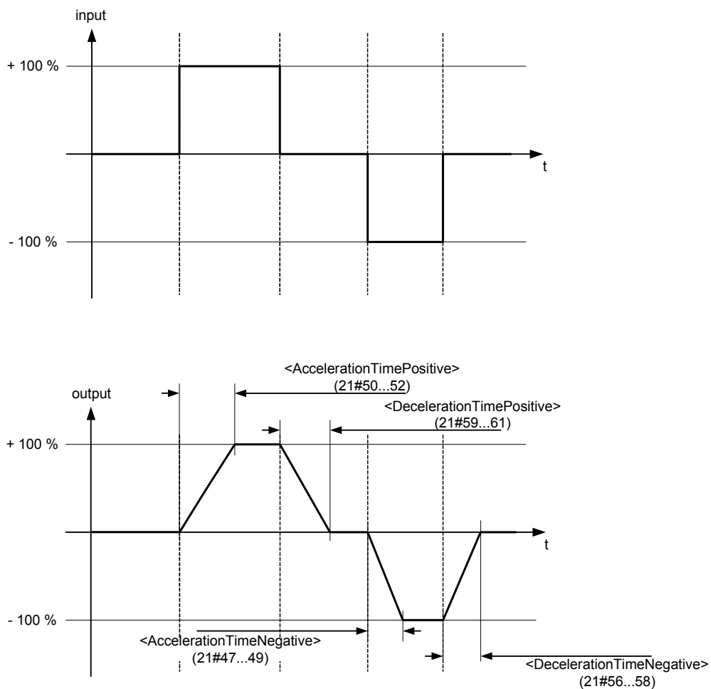
Figure 45: Ramp type 3
