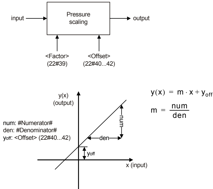
Figure 57: Scaling function
