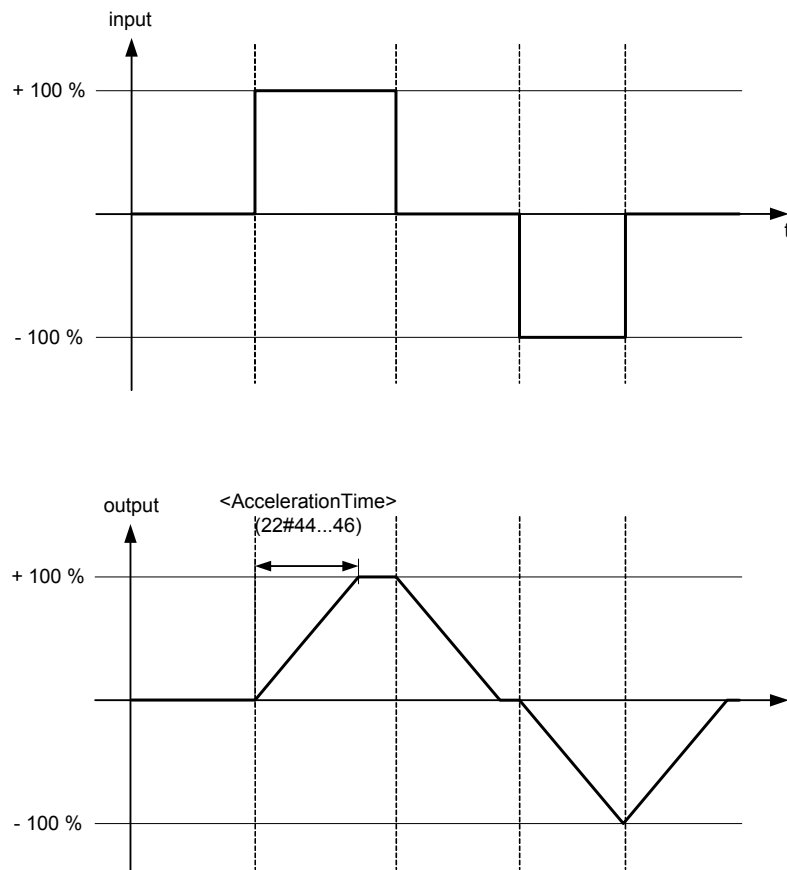
Figure 59: Ramp type 1
