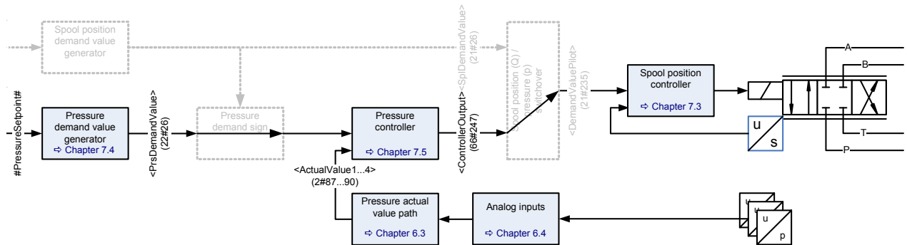
Figure 37: Pressure control closed loop
