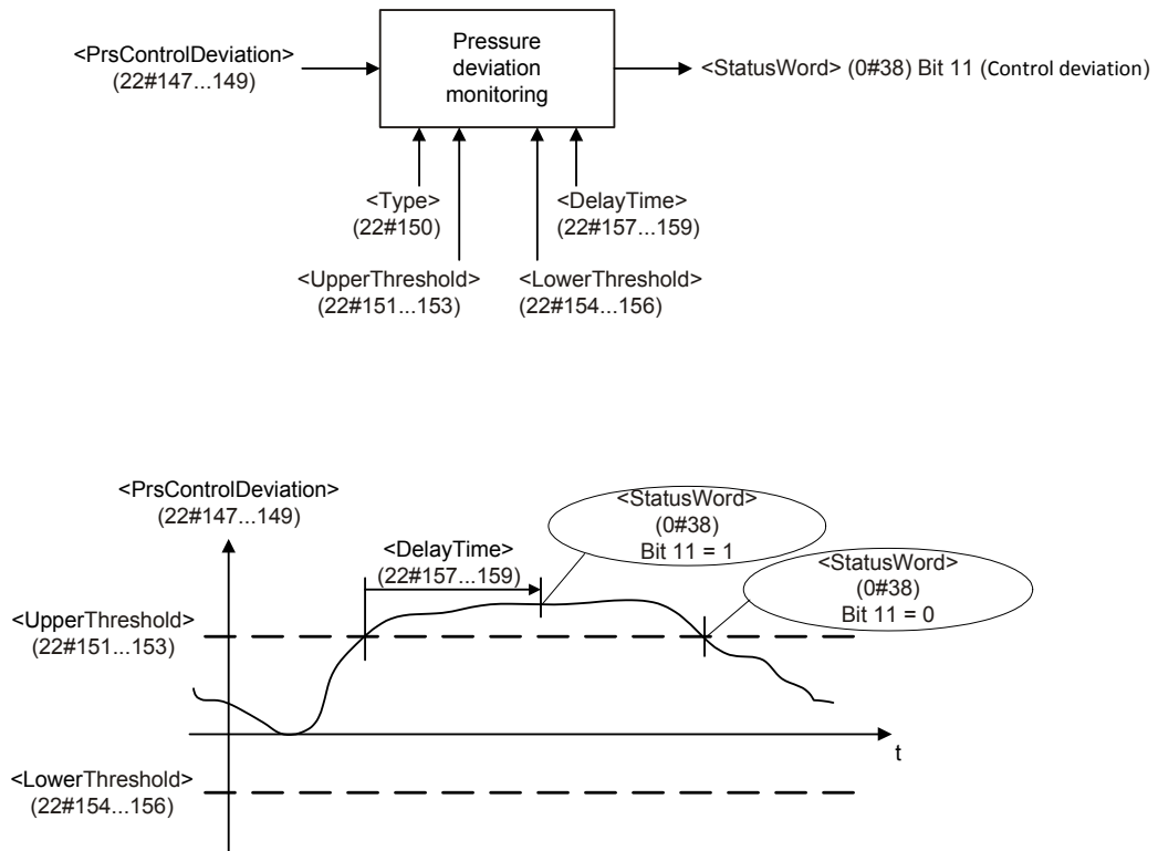
Figure 82: Pressure control deviation monitoring
