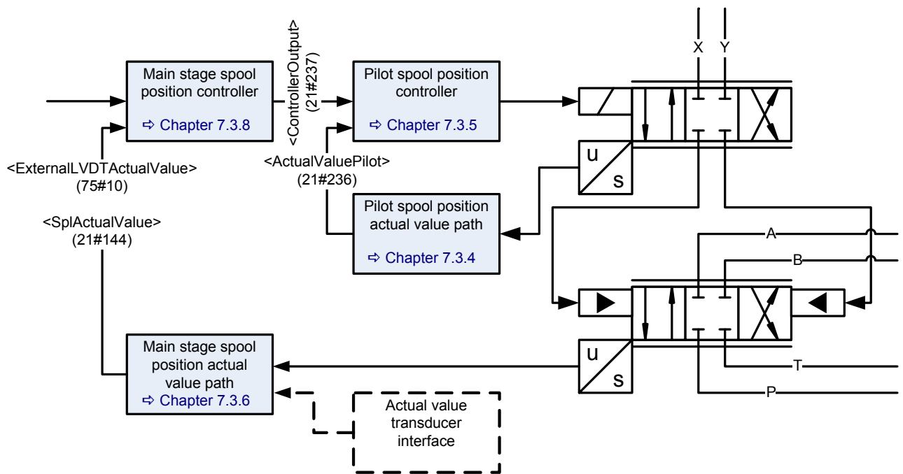
Figure 54: Dual stage servo valve for closed loop control
