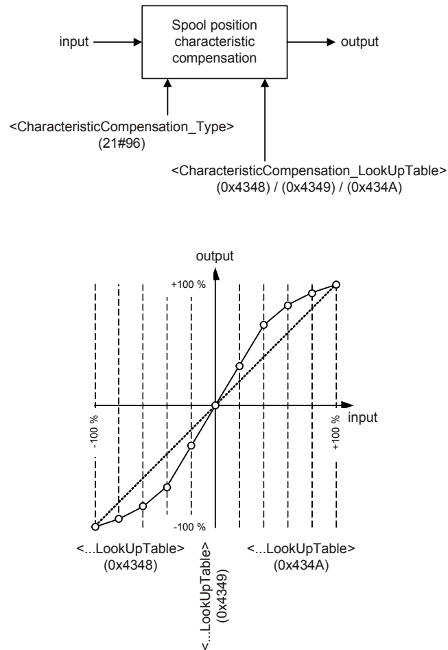
Figure 47: Characteristic compensation
