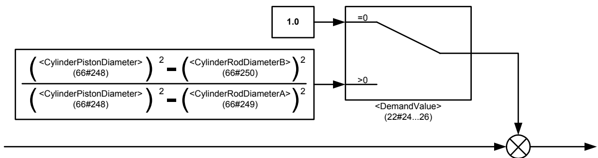
Figure 72: Alpha correction
