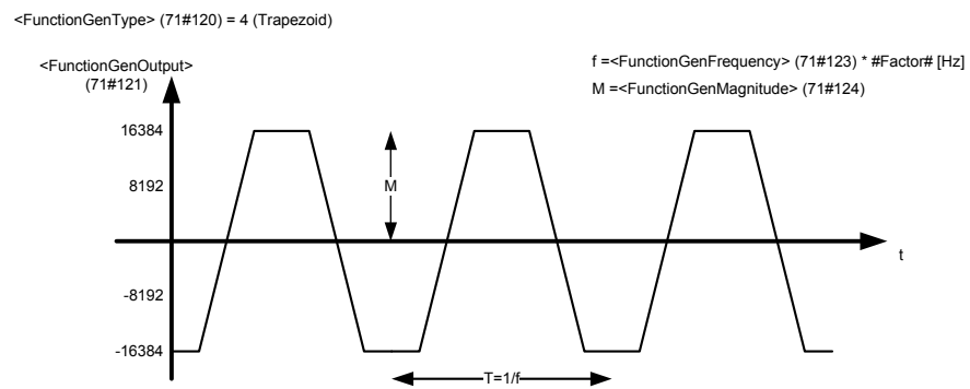
Figure 93: Trapezoid signal (type 4)
