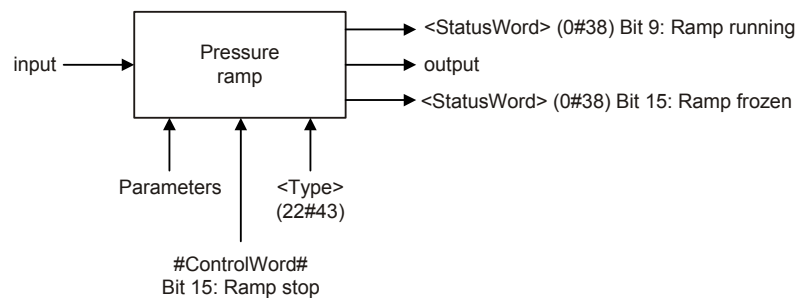
Figure 58: Ramp function
