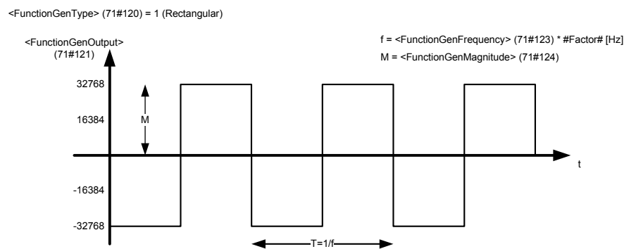
Figure 90: Rectangular output signal (type 1)
