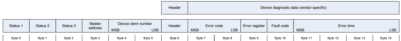
Figure 9: Device diagnostic data structure
