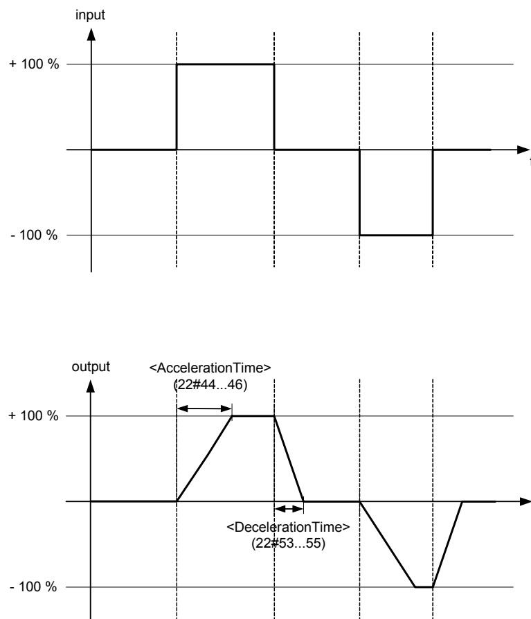
Figure 60: Ramp type 2
