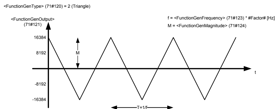
Figure 91: Triangle output signal (type 2)
