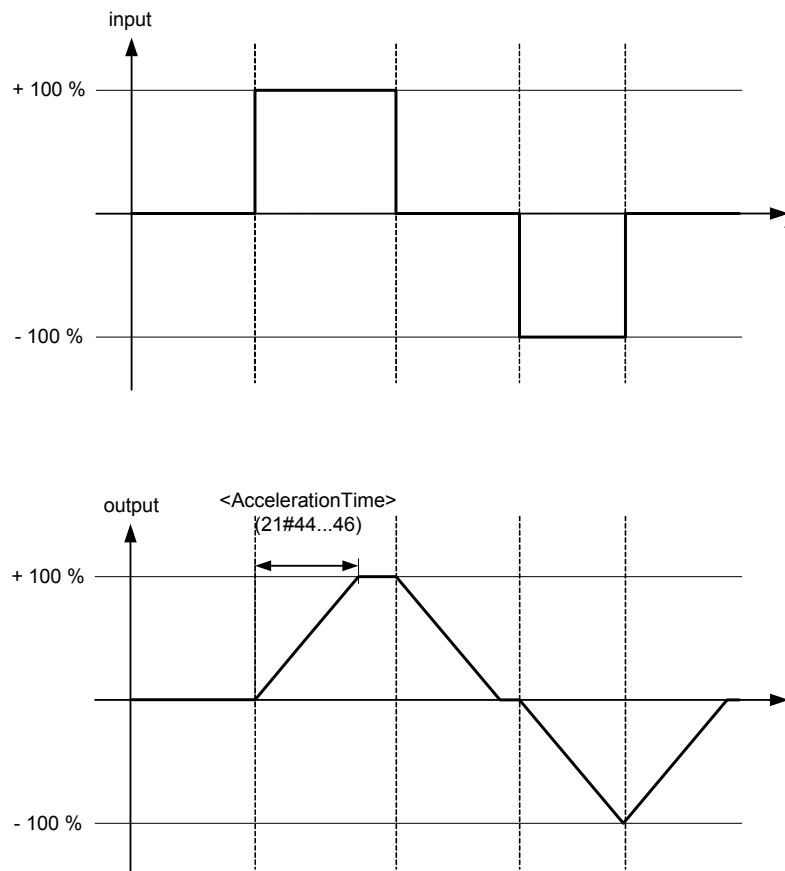
Figure 43: Ramp type 1
