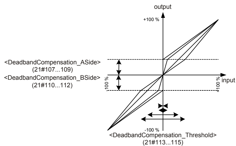
Figure 50: Dead band compensation type 2
