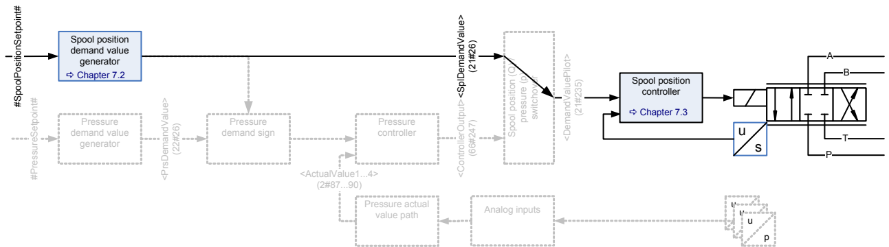
Figure 36: Spool position control closed loop for single stage and dual stage valves
