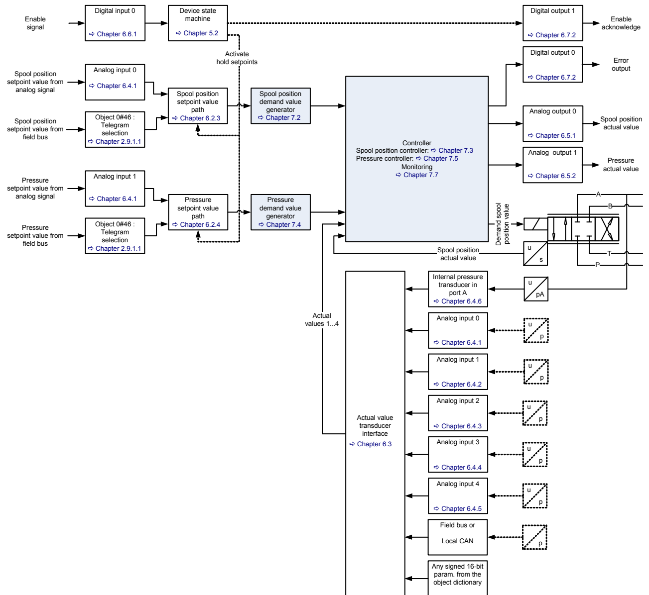
Figure 33: Servo valve controller and command signal conditioning
