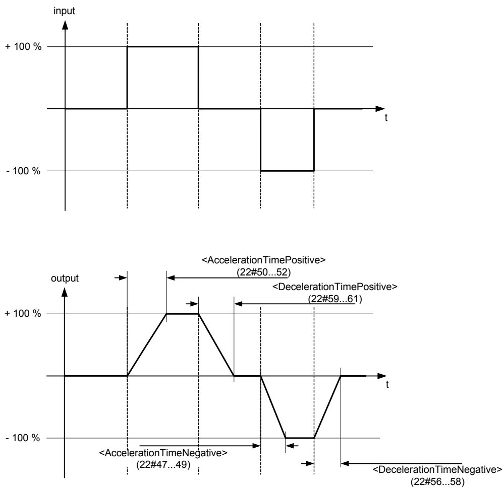
Figure 61: Ramp type 3
