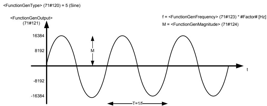
Figure 94: Sine signal (type 5)
