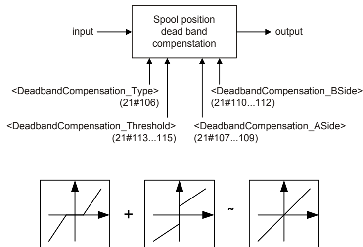
Figure 48: Dead band compensation
