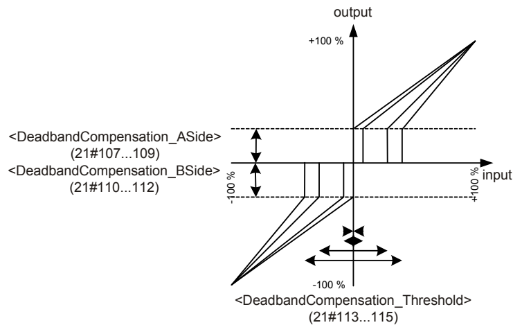
Figure 49: Dead band compensation type 1
