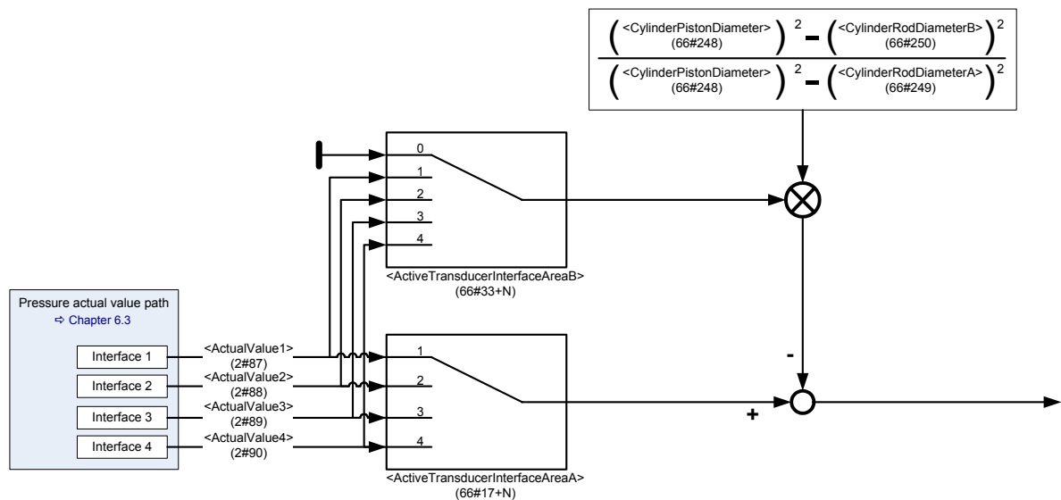
Figure 65: Pressure transducer selection
