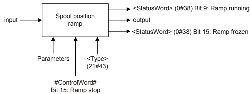
Figure 42: Ramp function
