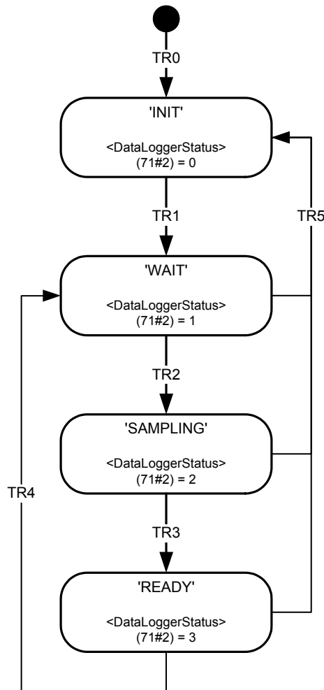
Figure 85: Data logger state machine
