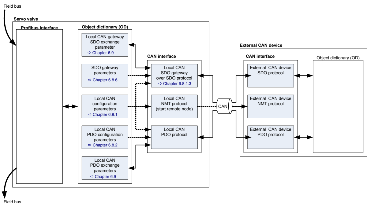
Figure 28: Structure of local CAN bus
