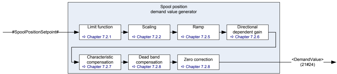
Figure 39: Spool position demand value generator
