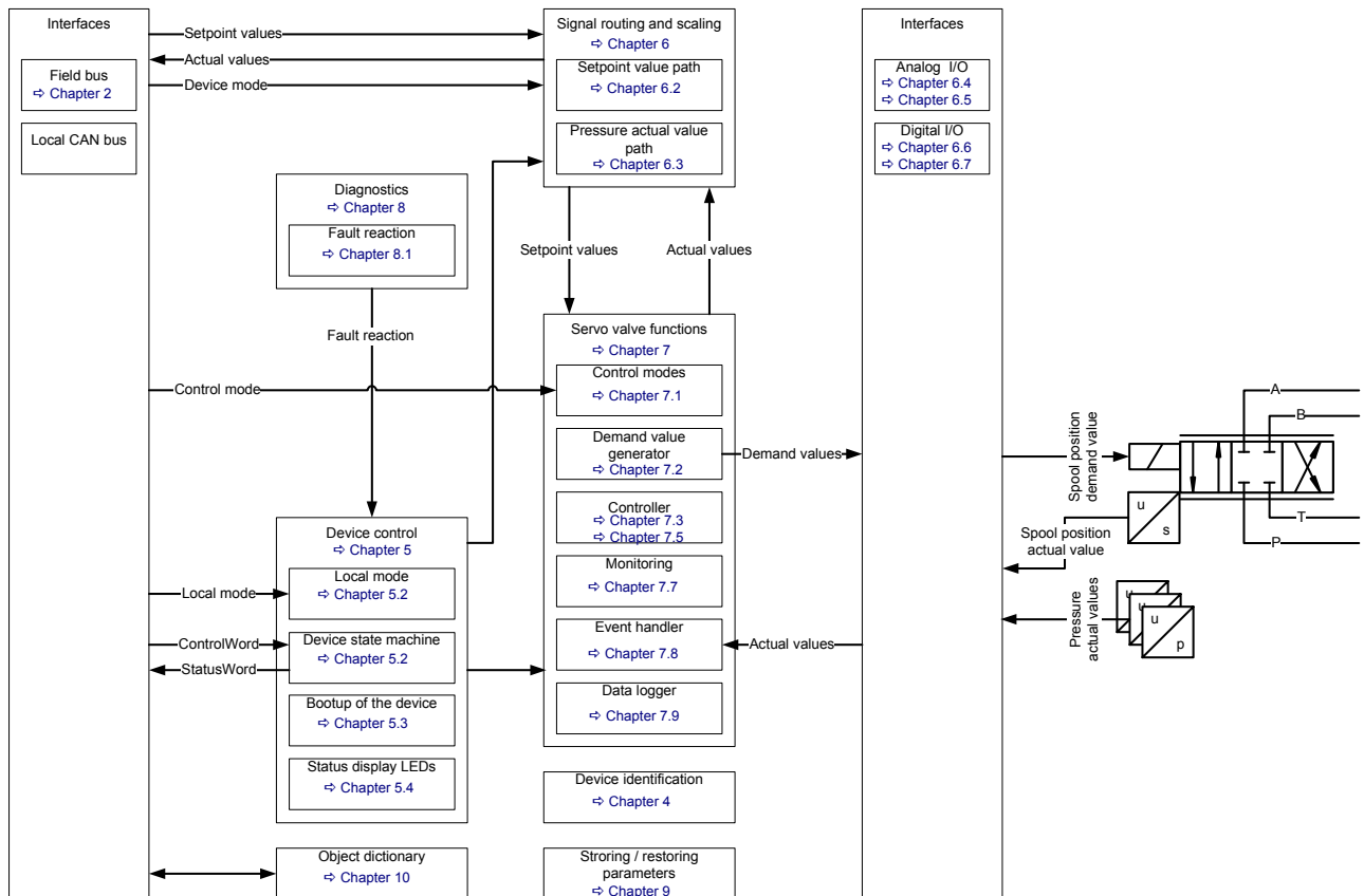
Figure 11: Device structure
