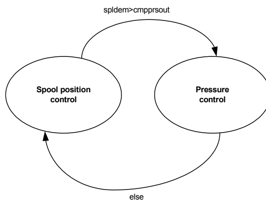
Figure 78: State machine used to switch between spool position control and pressure control
