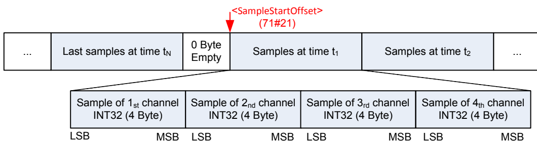
Figure 89: Data memory - four channels with INT32 parameters
