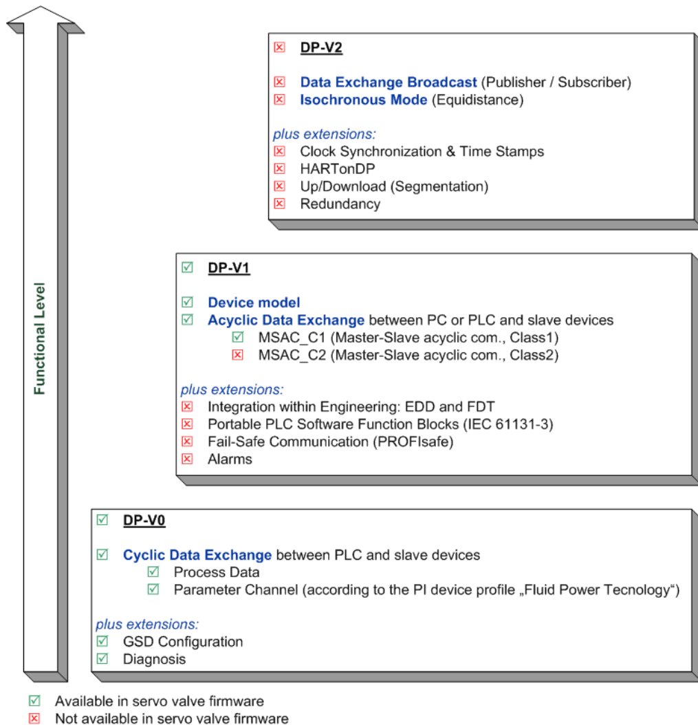
Figure 3: Profibus DP overview
