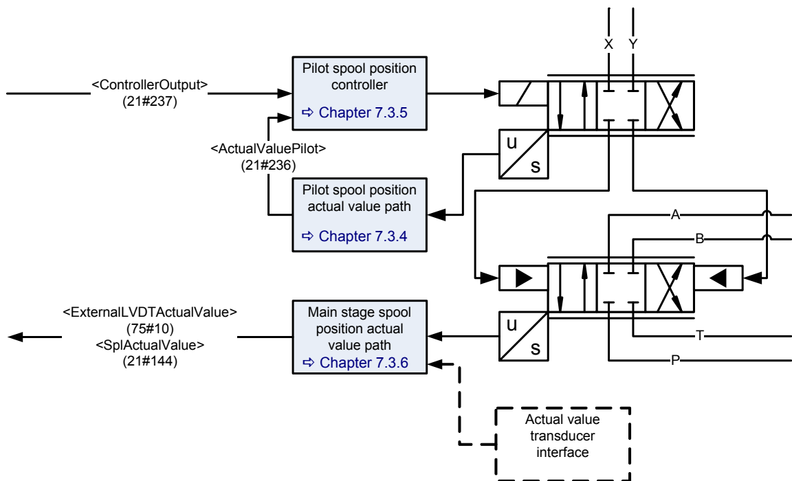
Figure 53: Dual stage servo valve for open loop control
