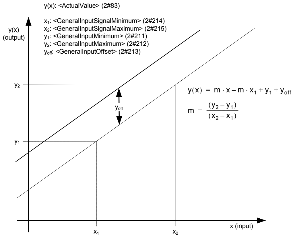
Figure 22: General input scaling
