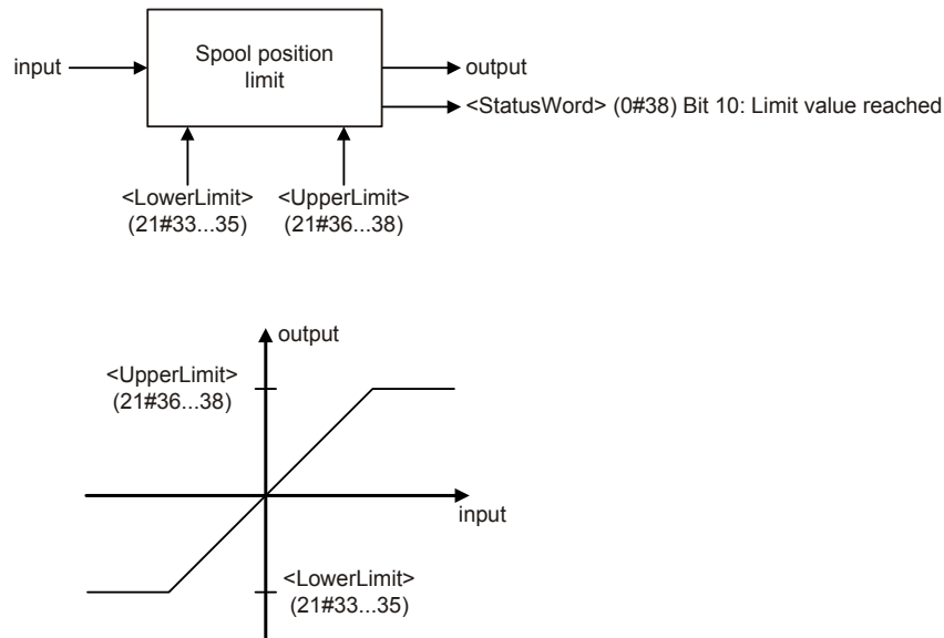
Figure 40: Limit function
