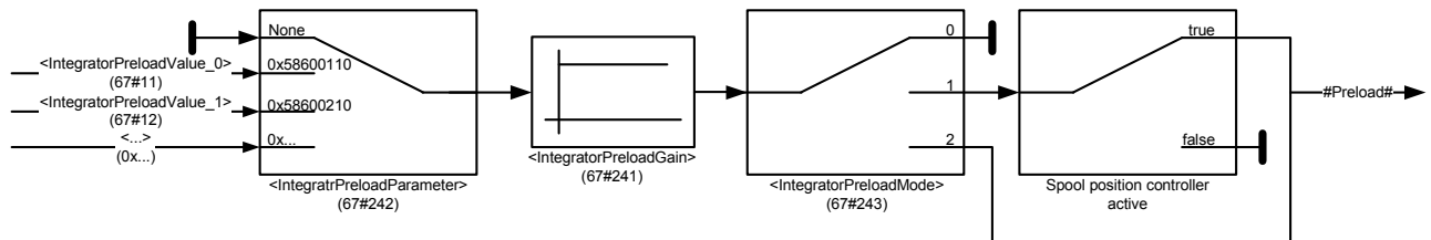
Figure 69: Integrator preload value
