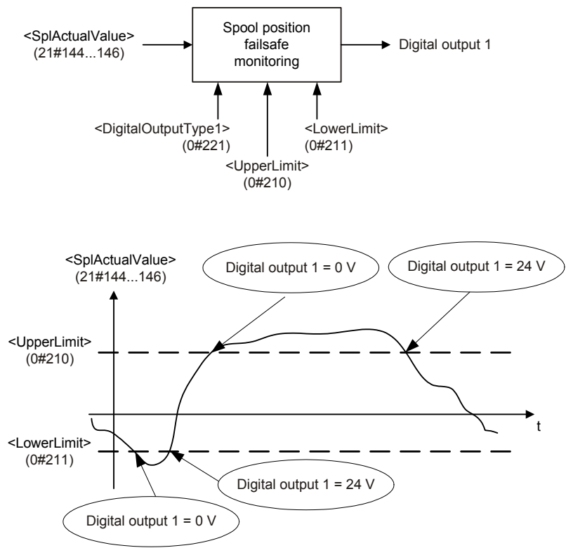
Figure 83: Failsafe monitoring
