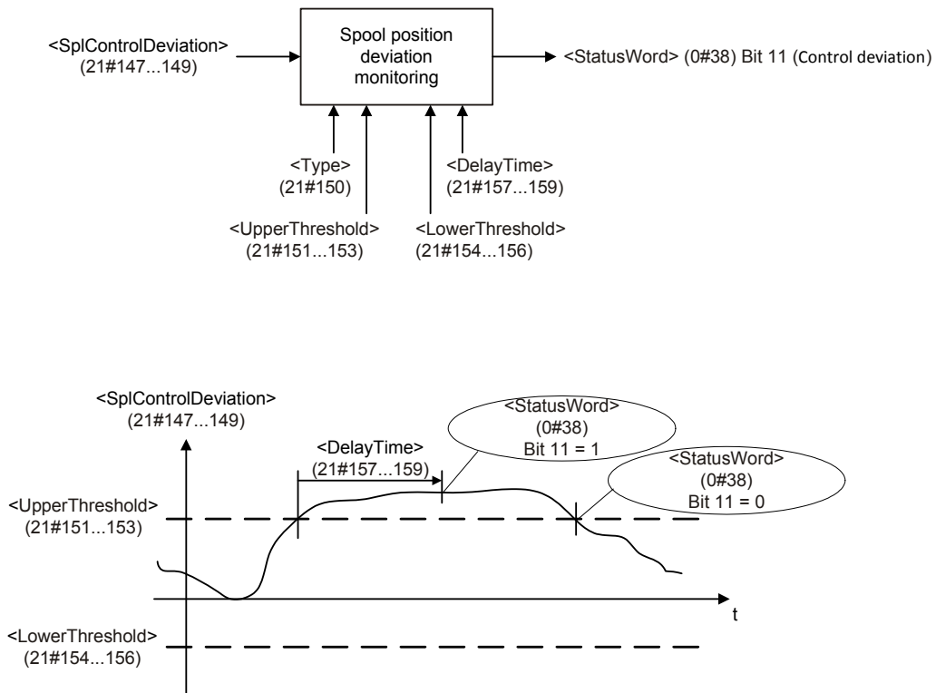
Figure 81: Spool position control deviation monitoring
