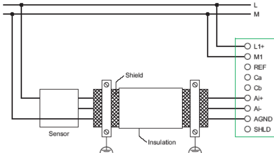
Connecting a Non-Isolated Analog Sensor (Voltage Signal) with the Same Auxiliary Energy Connection as the QAIO 2/2
