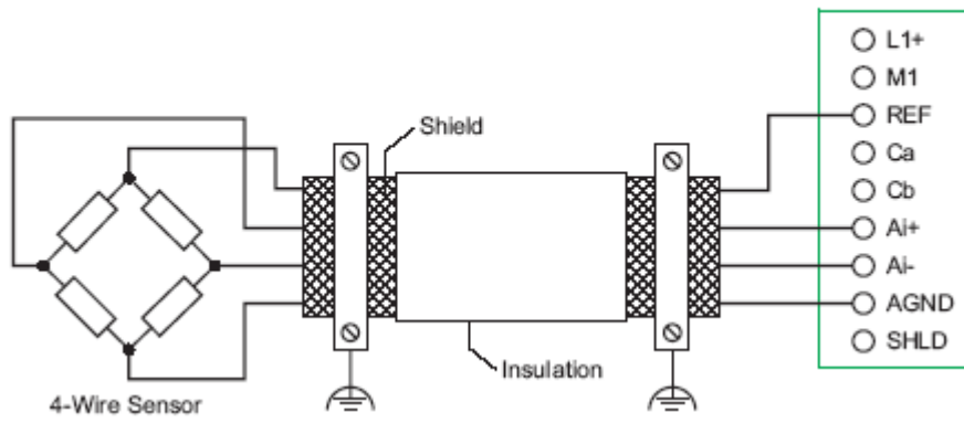
Connecting an Analog 4-Wire Sensor to the QAIO 2/2 Using the Internal Reference Voltage of the QAIO 2/2
