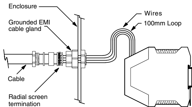
Preferred Wiring
