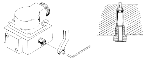
Figure 2 Mechanical Null Adjustment
