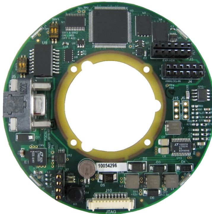
Figure 1-1: Model 923 Electronic Data Logger Card
