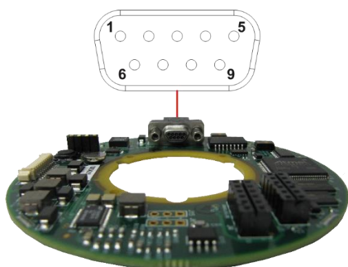
Figure 5-1: Micro-D (9-pin) Power & Data Connector (J5)
