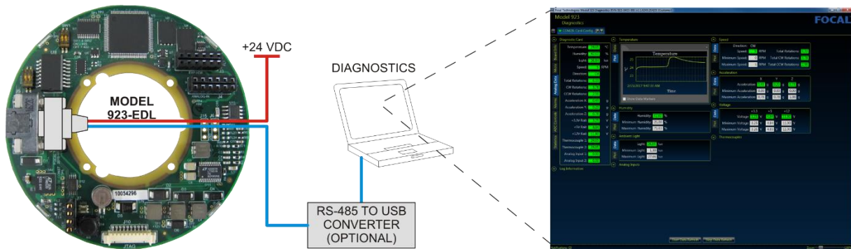
Figure 3-2: Model 923-EDL Typical Setup Connection Using a PC and Focal GUI
