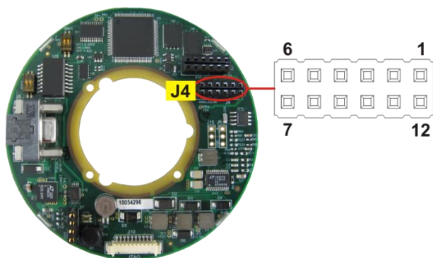
Figure 5-3: 12-pin Analog Input Connector (J4)
