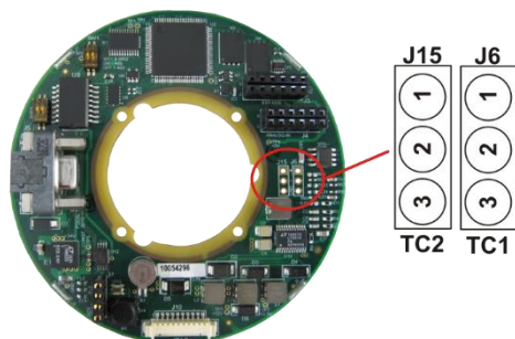
Figure 5-2: Thermocouple Input Connectors (J6, J15)
