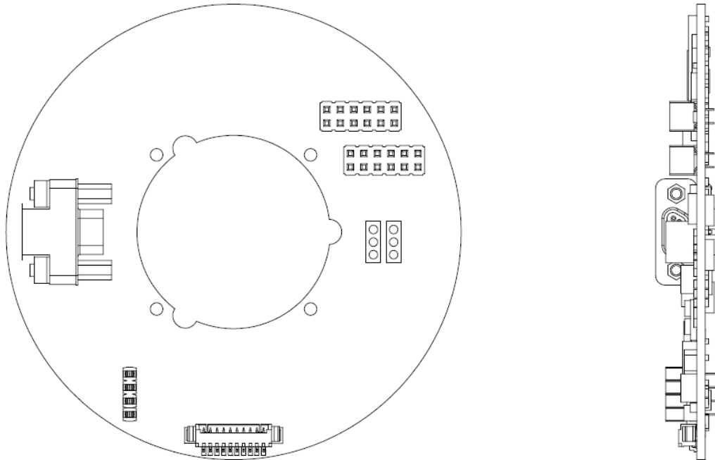
Figure 4-1: Model 923-EDL PCBA
