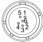
Media Converter Pin Numbers and Functions Shown - Mating Cable Plug Opposite
