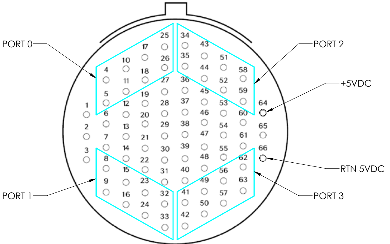
Front view of the J1 connector shown - mating cable plug opposite - see J1 D38999 Pin Function Chart for details
