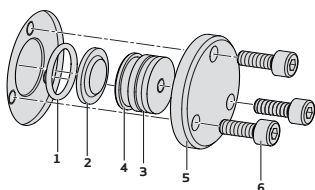
Fig.: Construction
