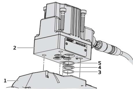
Fig.: Construction
