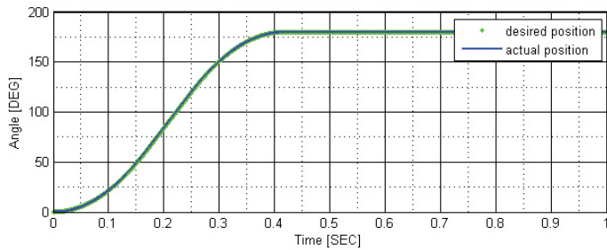
20 lb typical payload, no external disturbances:
