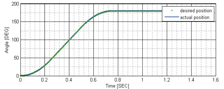
20 lb typical payload, full helicopter disturbance:
