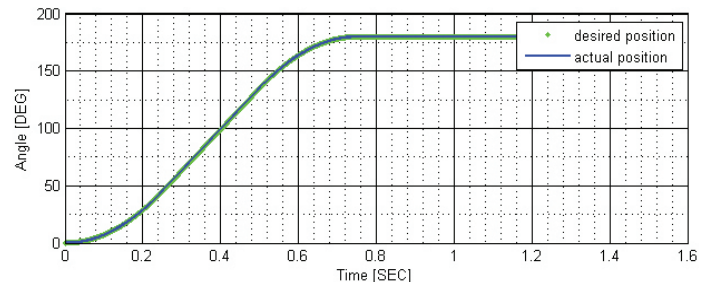
20 lb typical payload, half helicopter disturbance:
