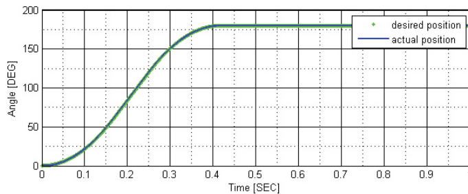
5 lb typical payload, no external disturbances:
