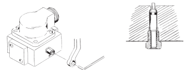
Figure 2 Mechanical Null Adjustment
